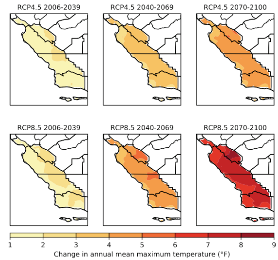
Change in annual mean maximum temperature (°F)
